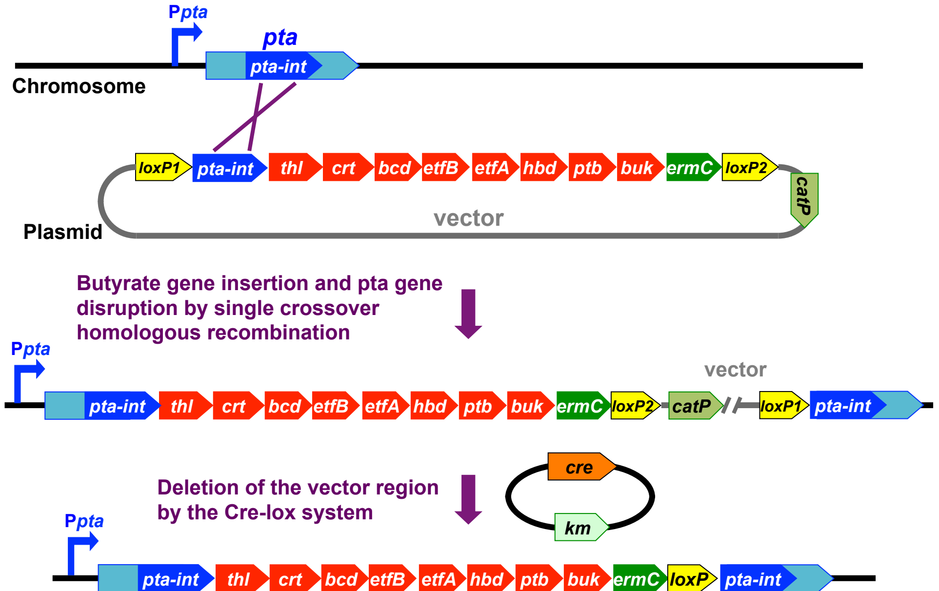
Figure S4. Construction of Strain B4.
