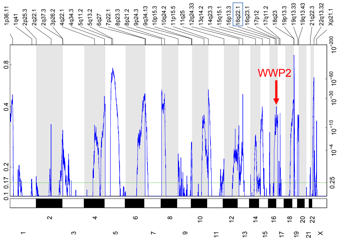
Fig. S3. GISTIC analysis of ovarian HGSC in TCGA dataset demonstrated significantly deleted sub-chromosomal regions. Vertical axis: GISTIC score (left) and q-value (right).
