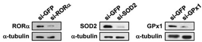
SUPPLEMENTARY FIG. S2. Effect of si-RNA duplexes on expression of genes. Primary cultures of rat hepatocytes were transfected with si-ROR \alpha , si-SOD2, or si-GPx1. Protein levels were measured by western blotting. GPx1, glutathione peroxidase 1; si-RNA, small interference RNA; SOD2, superoxide dismutase 2.
