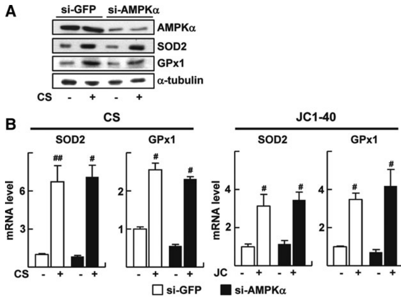
SUPPLEMENTARY FIG. S8. The CS-induced expression of SOD2 and GPx1 is not AMPK \alpha dependent. Primary rat hepatocytes were transfected with si-AMPK \alpha and then treated with 20 \mu M CS (A) or 50 \mu M JC1-40 (B) for 24 h. The protein- and mRNA-level were measured by western blotting and qRT-PCR, respectively. # p <0.05 and ## p <0.01 versus vehicle with si-GFP or si-AMPK \alpha . AMPK, AMP-activated protein kinase
