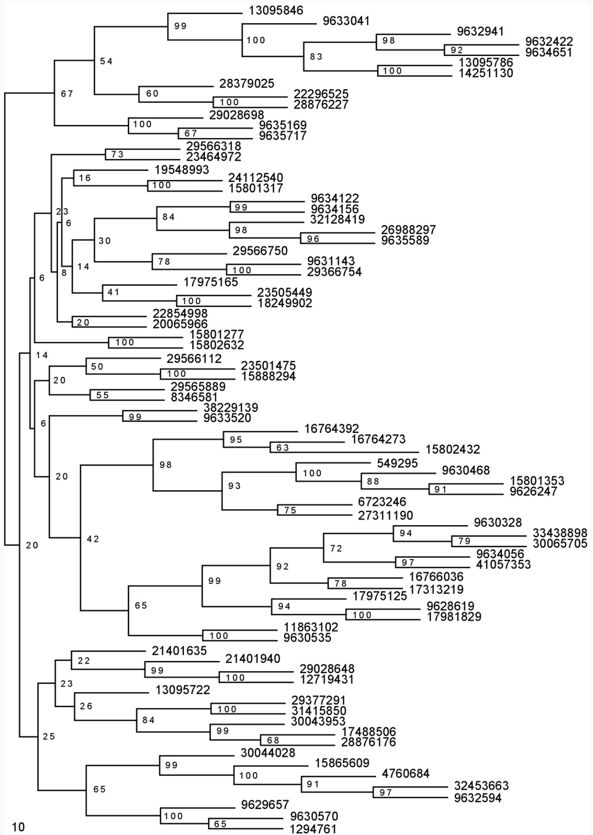
leaves are labeled with the gi number of the corresponding prohead protease
