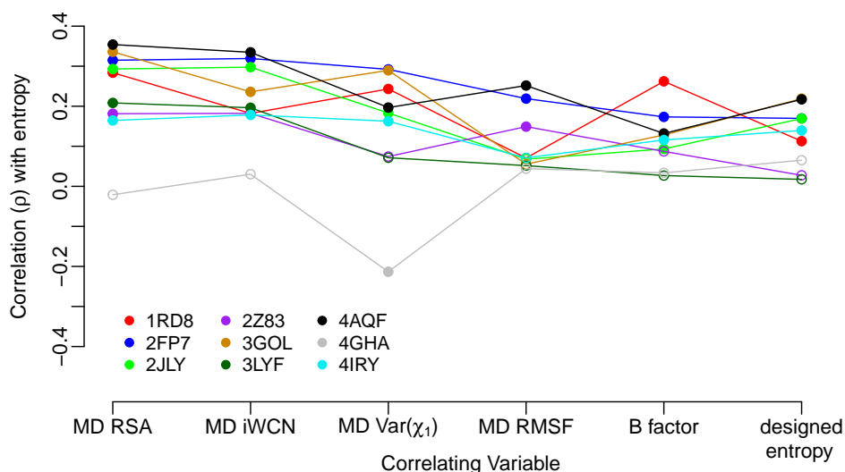
Fig. 2 Spearman correlation of sequence entropy with measures of buriedness, packing density, and structural flexibility, as well as designed entropy. Each symbol represents one correlation coefficient for one protein structure. Significant correlations ( P < 0.05 ) are shown as filled symbols, and insignificant correlations ( P \geq 0.05 ) are shown as open symbols. The quantities MD RSA, MD iWCN, MD \text{Var}(\chi_1) , and MD RMSF were calculated as time-averages over 15ns of MD simulations. B factors were obtained from crystal structures, and designed entropy was obtained from protein design in Rosetta. Compared to the measures of structural variability and to designed entropy, MD RSA and MD iWCN the buriedness measures consistently show stronger correlations with sequence entropy. Note that results for MD iWCN are largely identical to those for MD iCN, so only MD iWCN was included here.
