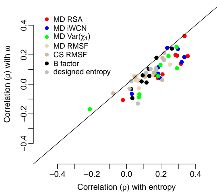
Fig. 5 Spearman correlations of structural quantities with sequence entropy and with the evolutionary rate ratio \omega . Nearly all points fall below the x = y line, indicating that structural quantities generally predict as much as or more variation in sequence entropy than in \omega .
