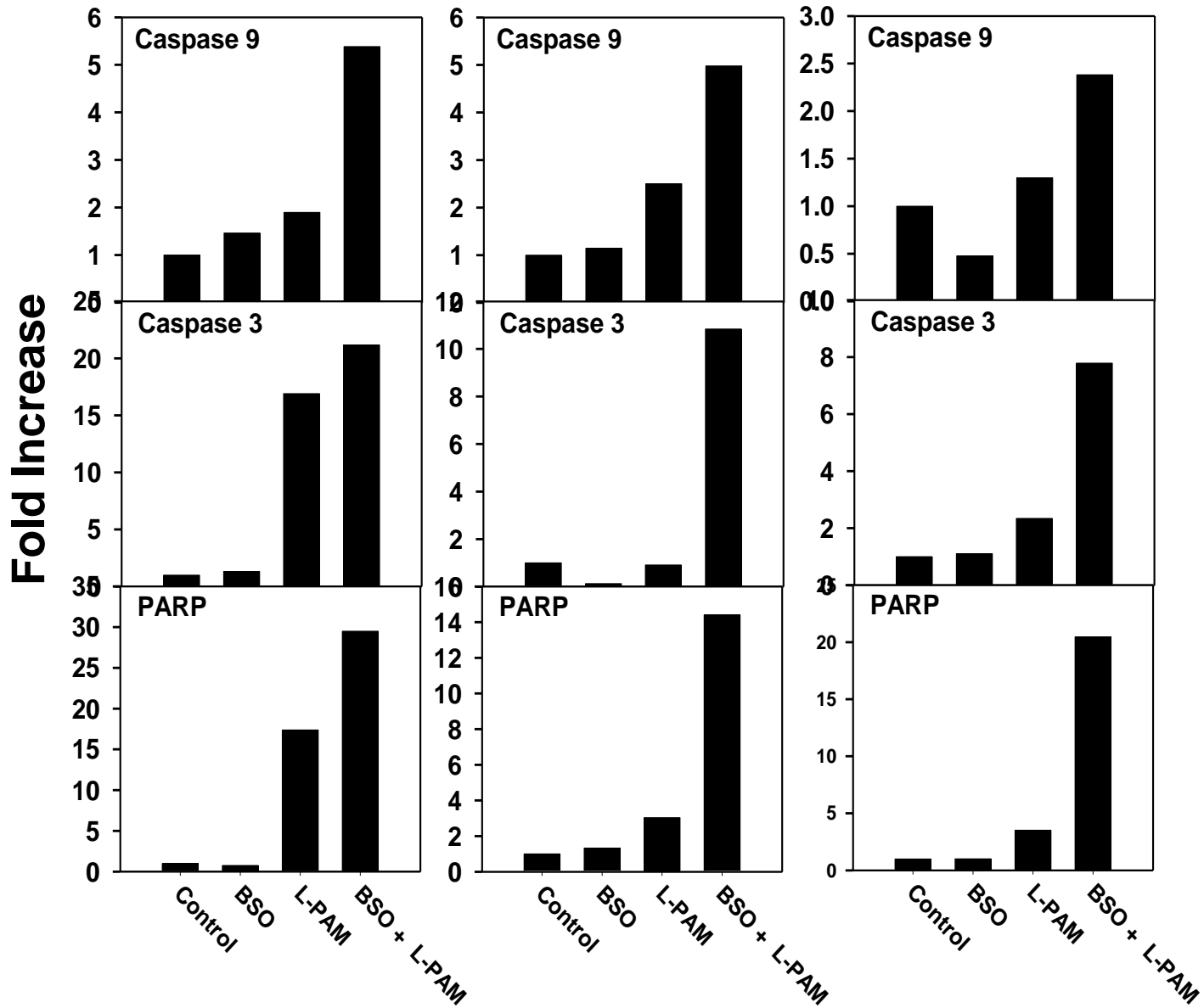
Supplementary Figure 3: Densitometry analysis of cleaved caspase and PARP as normalized by the total \beta -actin expression. Representative blots are shown in Figure 5a.
