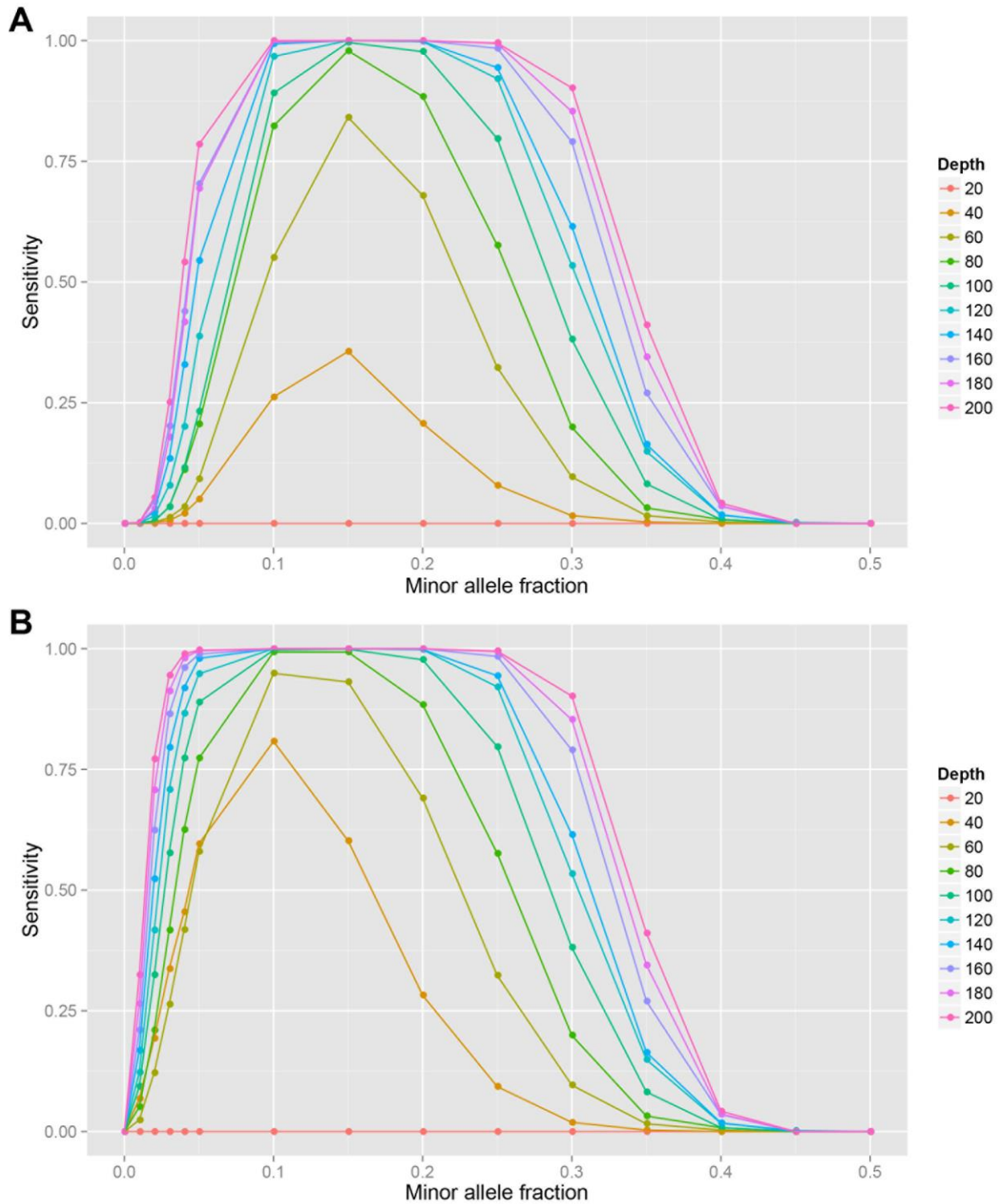
Figure S4. The theoretical sensitivity to identify postzygotic single-nucleotide mutations (pSNMs) with varied minor allele fraction, sequencing depth, and base quality. The base quality was set as 30 (A) and 60 (B). The sensitivity to detect pSNMs increased when either the sequencing depth or the base quality increased.
