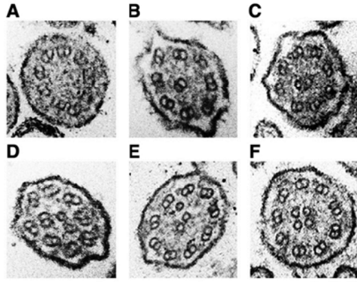
Supplementary information, Fig S2 Transmission electron microscopy images of the cross sections of axonemes in the tracheal epithelial cilia of CYLD knockout mice. (A) Absence of the central microtubule pair. (B) Absence of the central pair and transposition of an outer microtubule doublet. (C) Lacking an outer doublet. (D) Transposition of an outer doublet. (E and F) Extra central microtubules. Scale bars, 100 nm.
