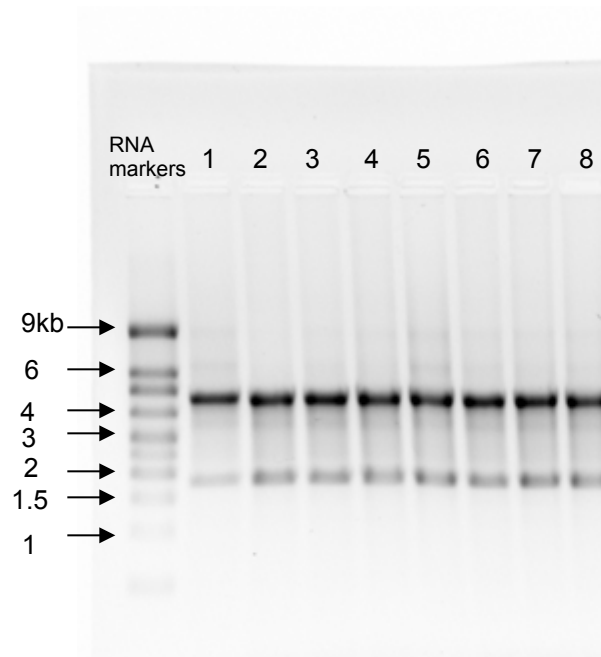
Figure S1. RNA gel demonstrating intact RNA samples. Native agarose gel electrophoresis was used to resolve the intact 28s and 18s rRNA bands. 2ug of RNA were run per lane.
