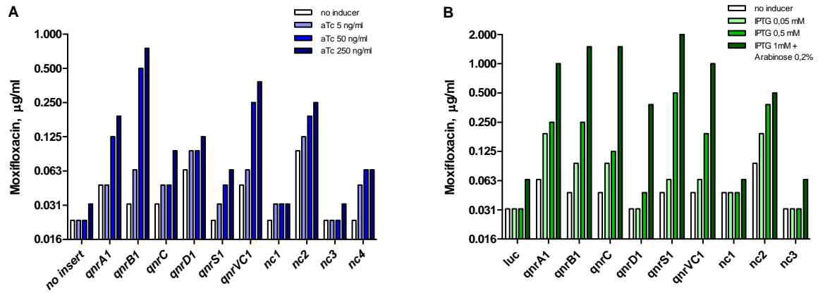
Figure S1. Moxifloxacin MICs for recombinant E. coli strains carrying known qnr genes or novel candidates ( nc1-4 ). The investigated genes are situated on pZE21 (A) or pZA14 (B), and expression was stimulated by adding indicated concentrations of the inducers aTc (A) or IPTG/Arabinose (B).
