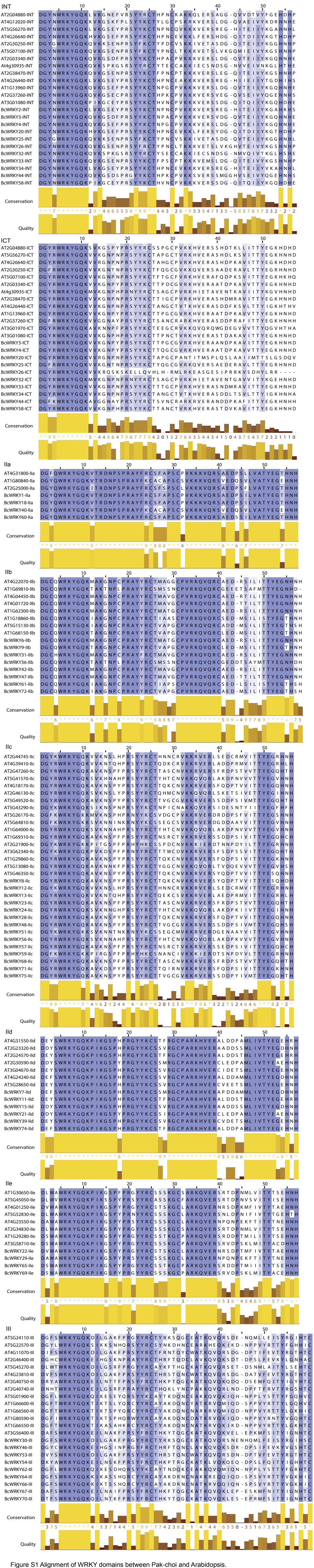
Figure S1 Alignment of WRKY domains between Pak-choi and Arabidopsis.
