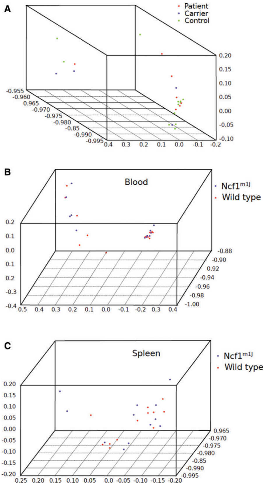
SUPPLEMENTARY FIG. S2. Principal component analysis (PCA) of all samples that were subjected to genome-wide gene expression profiling. PCA of the human samples is presented in (A), mouse blood samples in (B) and mouse spleen samples in (C).
