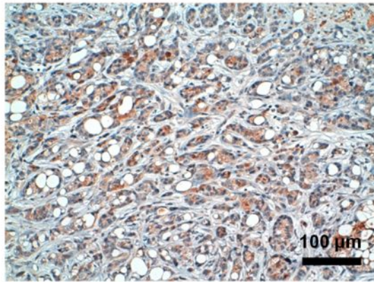
Mucin 5ac
