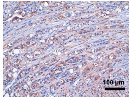
Somatostatin
