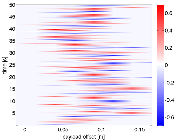
Figure 1: Intensity of the feedback signal of an inner spring as a function of the payload position relative to the center of mass and time during a single 50s run.
