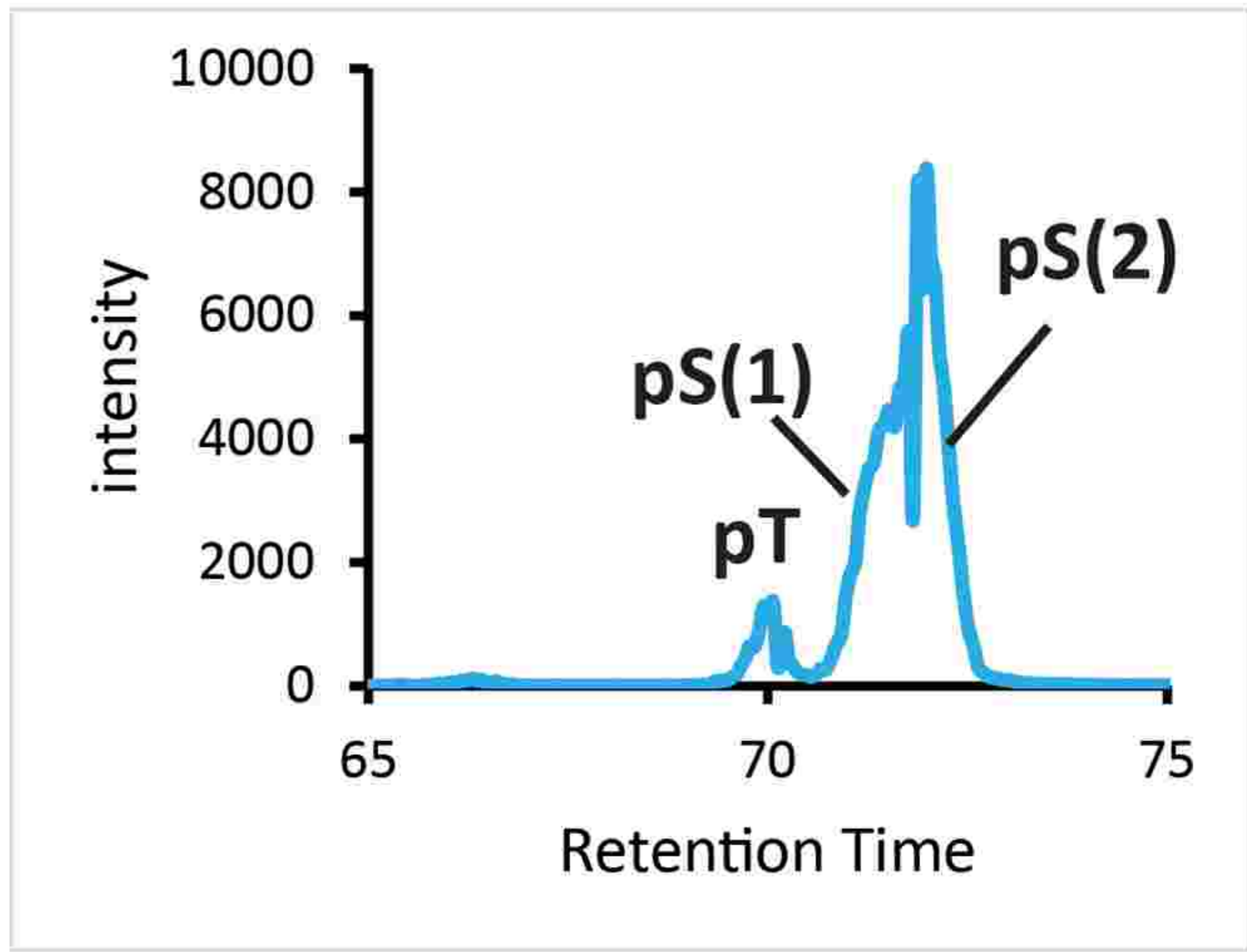
Cyclin C-CDK3
