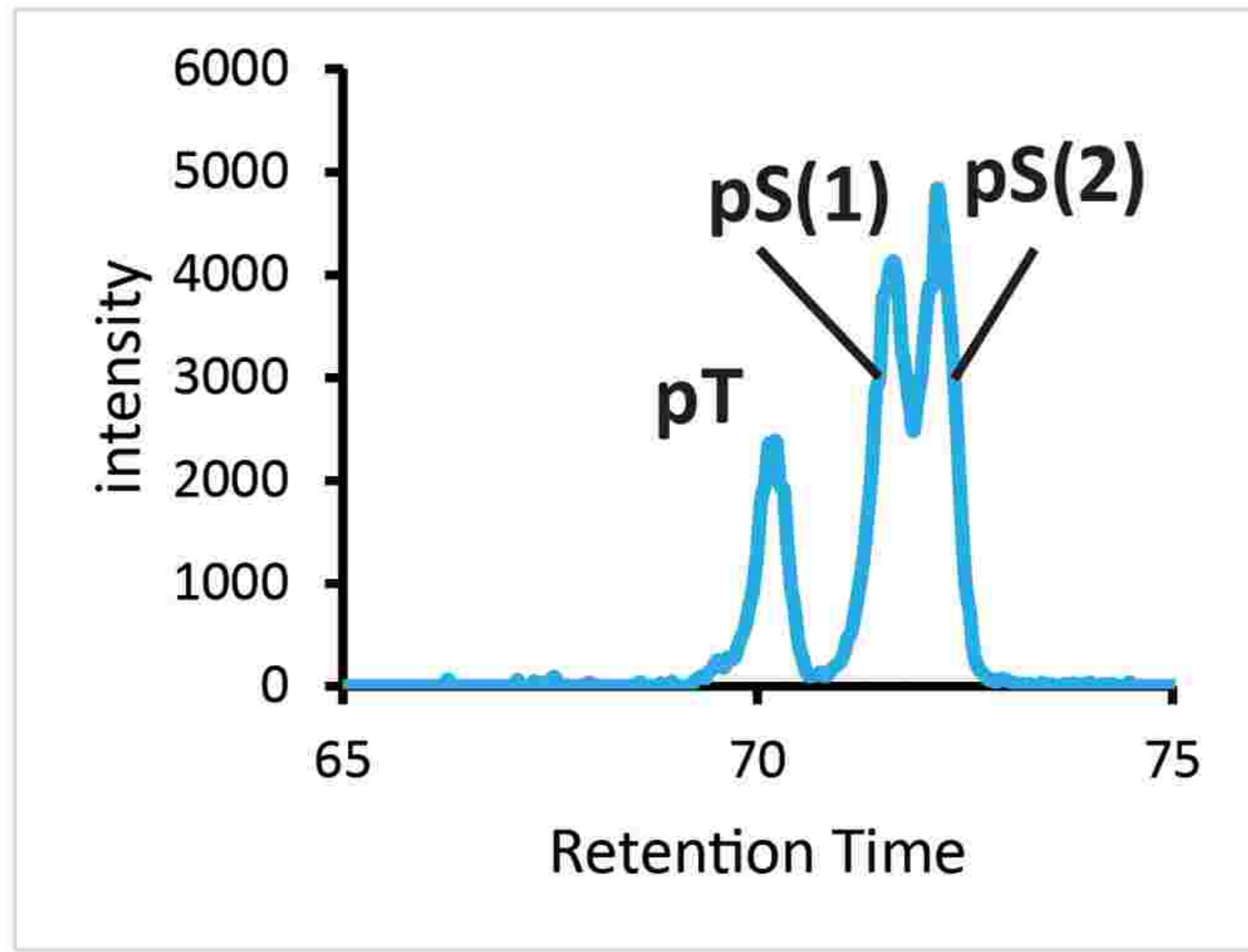
Cyclin C-CDK19
