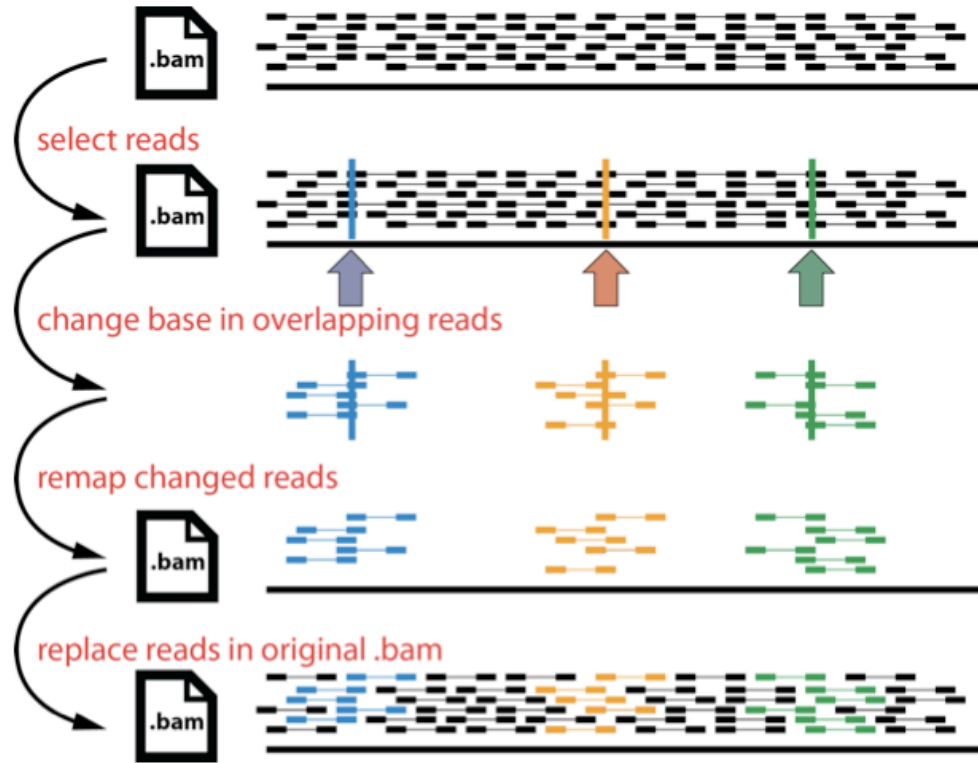
Figure S2: Diagram of bamsurgeon methodology. Mutations are spiked into BAM files by selecting locations with adequate coverage, extracting the reads, and adjusting the VAF according to the desirable VAF distribution. Once the bases in the reads are changed, the reads are remapped to the genome, replacing the reads in the original BAM file.
