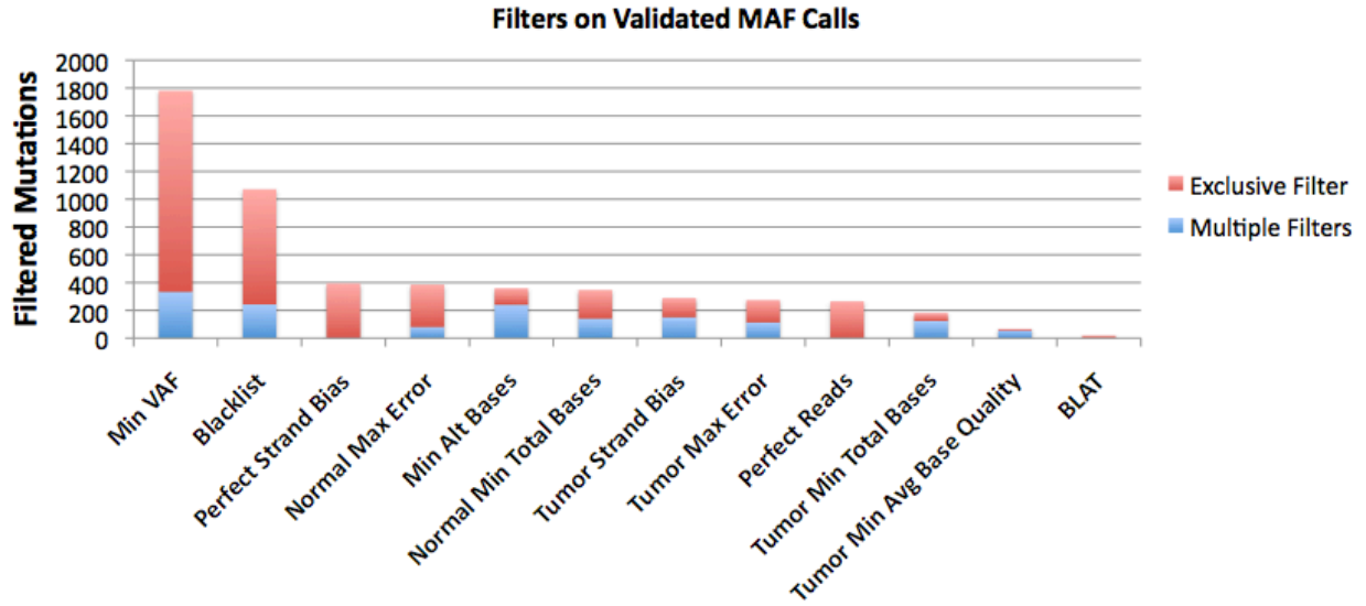
Figure S6: Filters applied to the RADIA mutations that validated as somatic in the endometrial TCGA MAF file. Thirty-three percent of the mutations had a DNA VAF of eight percent or less while 23% landed in blacklist regions that were ignored.
