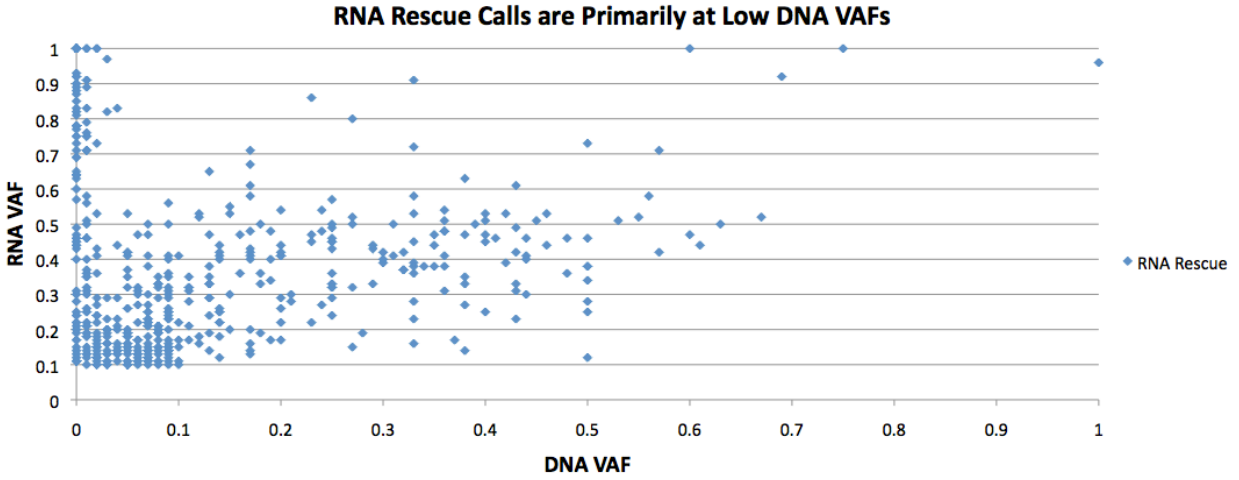
Figure S7: RNA Rescue calls are primarily at low DNA VAFs. RNA Rescue calls are primarily found at low DNA variant allele frequencies, but they also occur at higher frequencies where they were filtered due to non-depth related artifacts (e.g. strand-bias).
