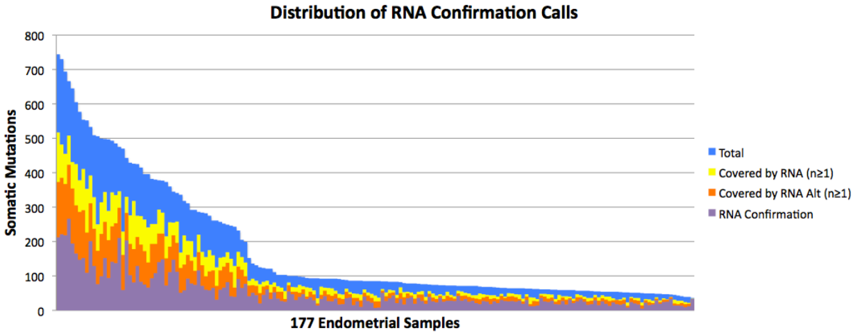
Figure S8: Distribution of RNA Confirmation Calls. The total number of mutations (blue) that are covered by at least one RNA read (yellow), one RNA read supporting the alternative allele (orange), and RNA Confirmation mutations with high support in both the DNA and RNA (purple).
