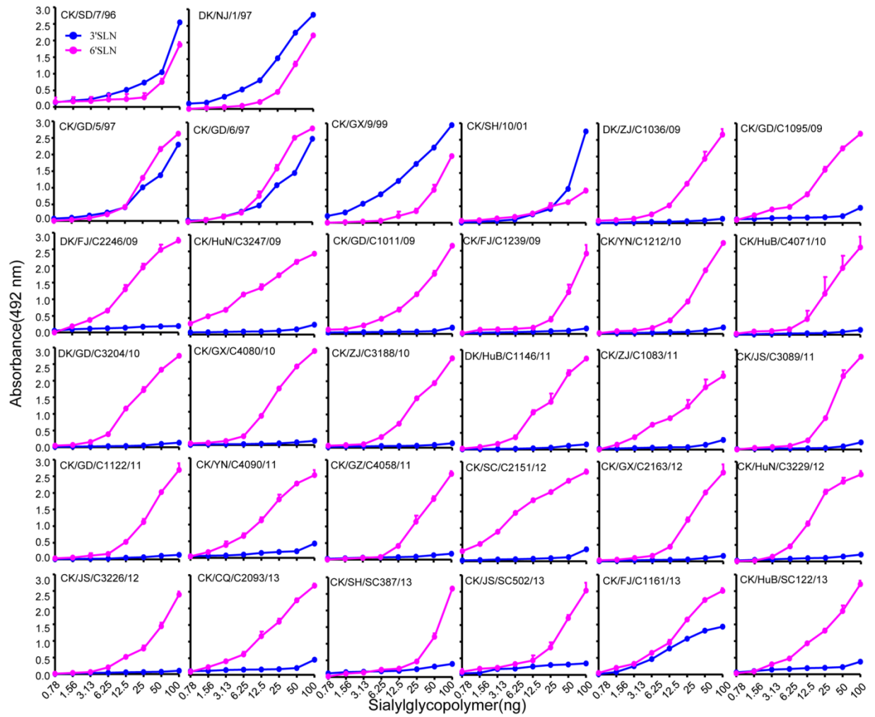
Figure S3. Characterization of the receptor-binding properties of H9N2 viruses. The binding of the viruses to two different biotinylated glycans ( \alpha -2, 3 glycan, blue; \alpha -2, 6 glycan, pink) was tested. The data shown are the means of three repeats; the error bars indicate the standard deviations.
