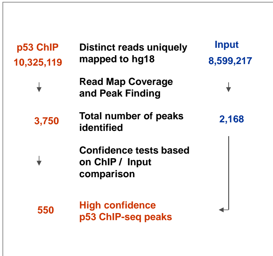
Figure S2. Defining high-confidence p53 ChIP-seq peaks in HCT116.
