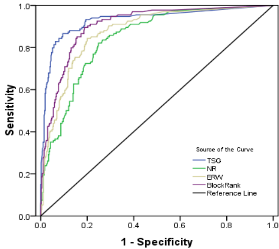
(e) ROC Curve - Alzheimer Disease
