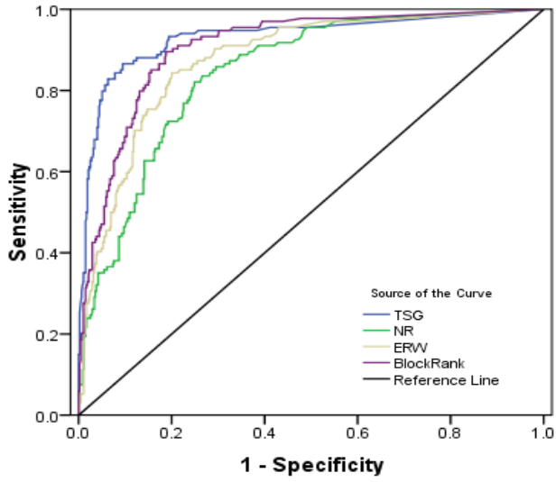
(c) ROC Curve - Prostate Cancer
