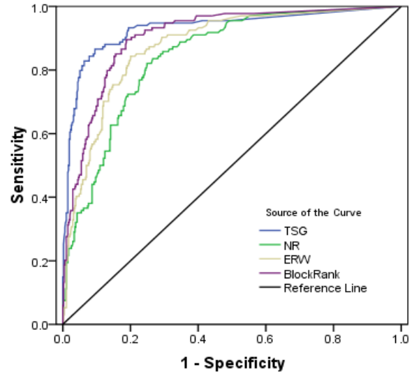
(b) ROC Curve - Lung Cancer
