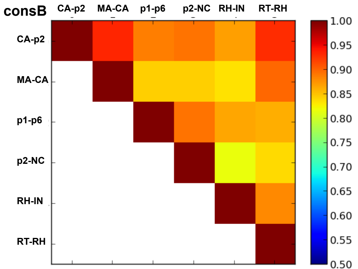
Figure 9 - Similarities of the active site cleft of PR in complex with different substrates
