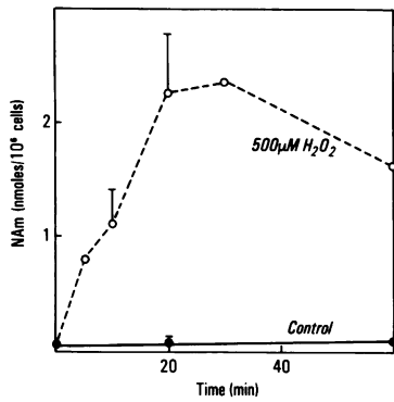
Figure 3. The effect of H_2O_2 on nicotinamide in the extracellular medium. 5 \times 10^6 cells/ml were incubated at 37^\circ C in MGB in the presence ( \circ ) or absence ( \bullet ) of 500 \mu M H_2O_2 . Samples of supernatant were prepared as described in Methods and nucleosides were separated and quantitated by HPLC. Each point represents the mean of two experiments. Error bars show standard deviations for n = 3 .
