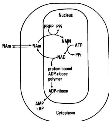
Figure 11. Synthetic and catabolic steps of poly-ADP-ribose metabolism. NA , nicotinamide; NMN , nicotinamide mononucleotide; PRPP , phosphoribose pyrophosphate; PPI , pyrophosphate; RP , ribose phosphate.
