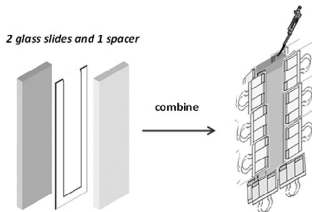
SUPPLEMENTARY FIG. S1. Apparatus for making 2D hydrogel surface.
