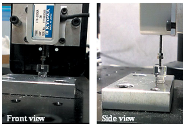
SUPPLEMENTARY FIG. S3. Experimental setup of load cell ( top ) and hydrogel ( bottom ).
