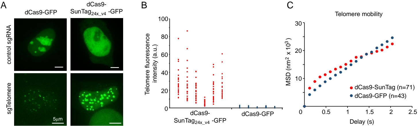
Figure S4 - related to figure 5. dCas9-SunTag can recruit many copies of scFv-GCN4-GFP to a genomic locus.
