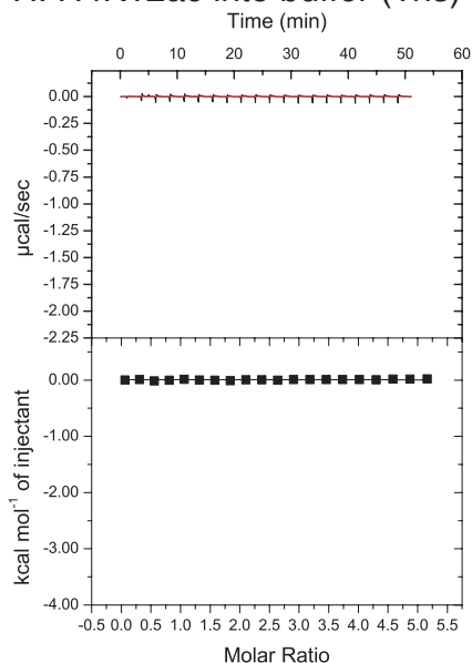
H. H4K12ac into buffer (Tris)
