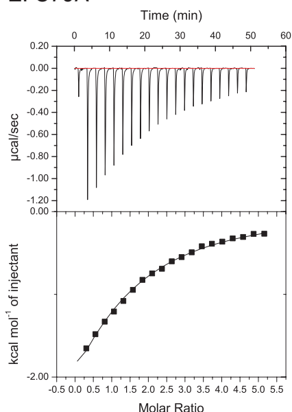
H. H4K12ac into buffer (Tris)
