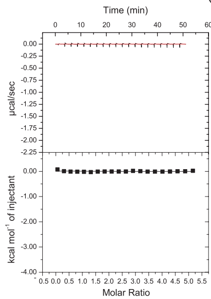
H. H4 unmodified into buffer (Tris)
