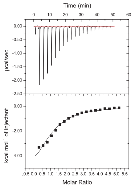
H. H2AK5ac into buffer (Tris)
