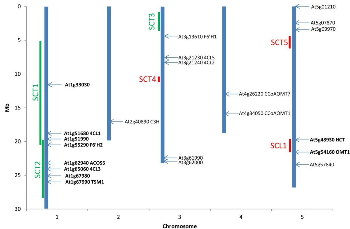
Figure S1. The position of known loci involved in scopolin and scopoletin biosynthesis. Mapped QTLs are highlighted in green and red colours. QTLs characterized by the highest LOD score values are highlighted in red. Loci co-localizing with QTLs are highlighted in bold.
