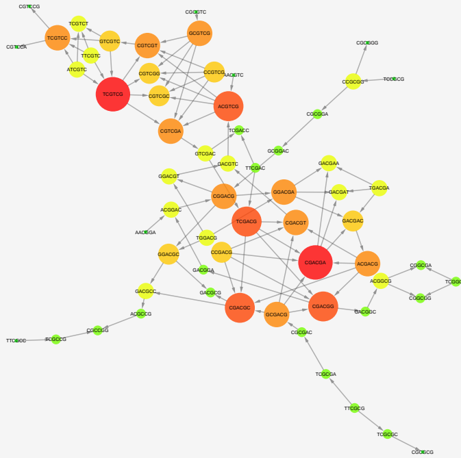
Figure S1: An example of the weakly connected component for ESEs where R=100 . The vertex color and size is relative to its degree.
