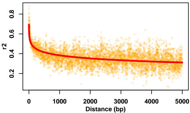
Chr3
