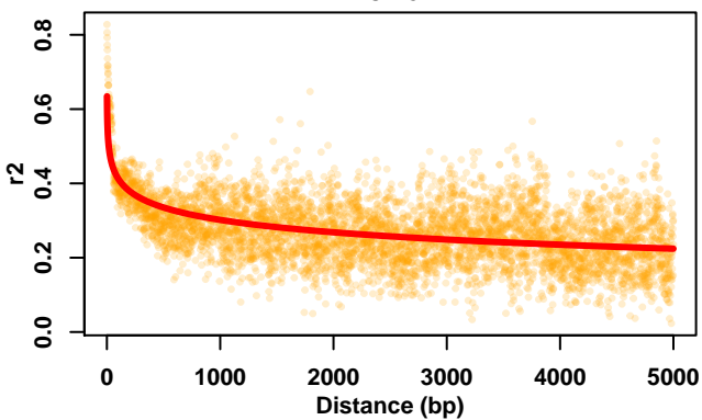
Chr5
