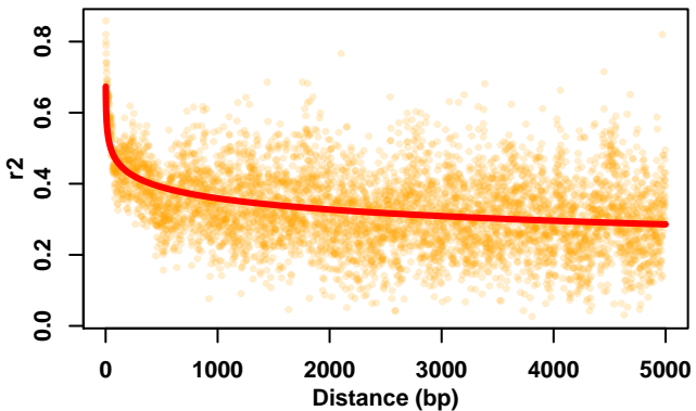
Chr7
