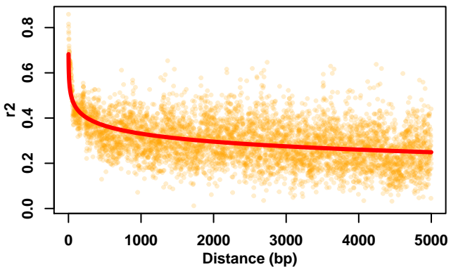
Chr9
