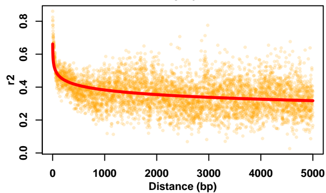
Chr6
