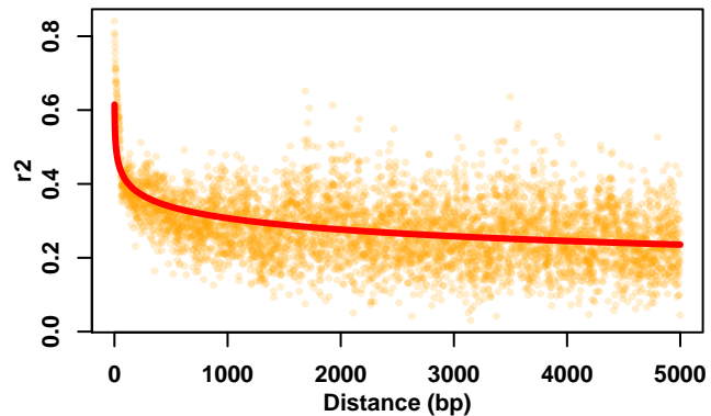
Chr8
