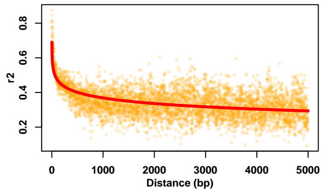
Chr2
