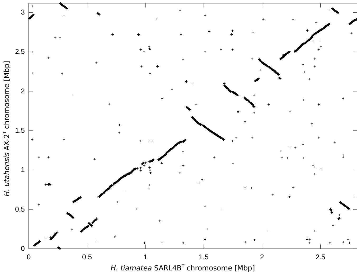
Fig. S1. Whole genome alignment between H. utahensis and H. tiamatea . The genome of H. tiamatea was split into 50 bp fragments and subsequently mapped on the H. utahensis with SSAHA2 v. 2.5 (Ning et al. , 2001).
