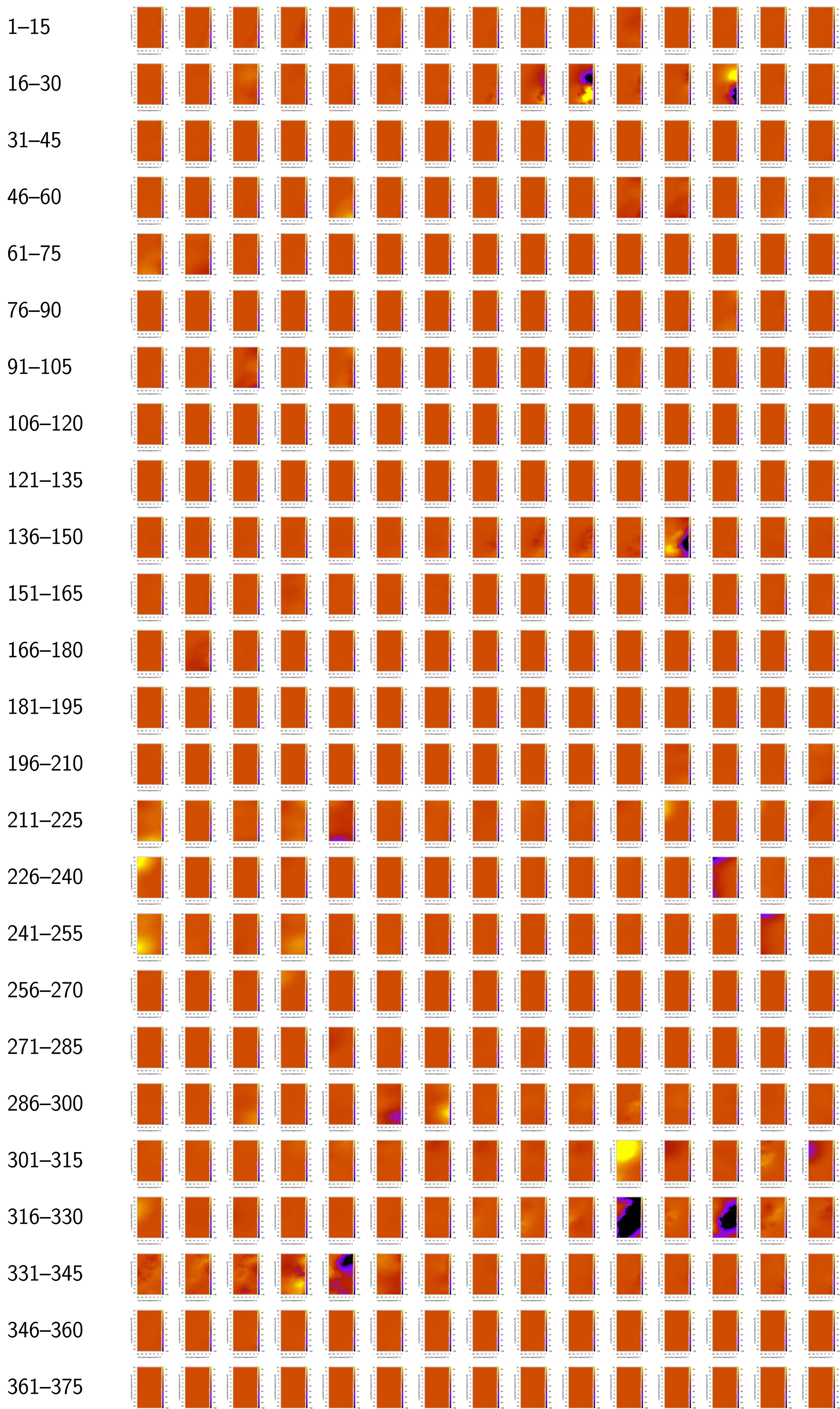
Figure S2. Energy landscapes showing contributions of all individual actin residues to the interaction of actin and tropomyosin, with the interaction energy noted by color level as in Figure 2.
