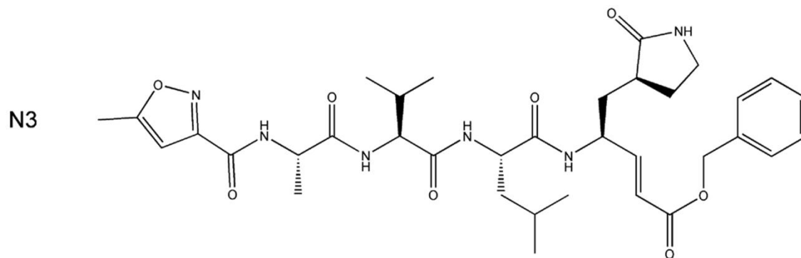
Figure S1 Chemical structure of the compound N3.
