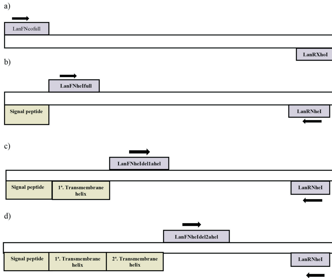
Figure S1 - Schematic representation of the positions of the primers used to amplify the DNA sequences and lanosterol 14 \alpha demethylase cDNA. (A) Primers LanFNcoIfull + LanRXhoI, (B) LanFNheIfull + LanRNheI, (C) LanFNheI del1ahel + LanRNheI and (D) LanFNheI del2ahel+ LanRNheI.
