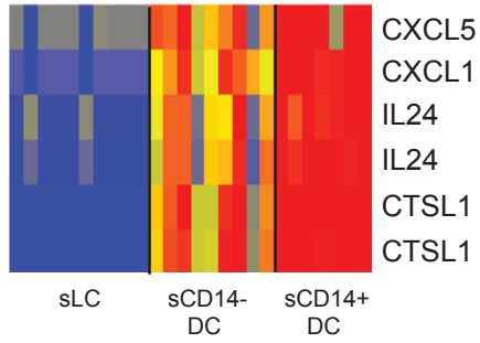
Figure S5: 6 transcripts representing 4 genes differentially expressed between the 3 skin DC subsets. a. Hierarchical clustering of the 6 transcripts differentially expressed in the 3 skin DC subsets. b. Bar charts representing the mean raw expression value for 4 of the 6 transcripts. Bars represent the standard deviation.
