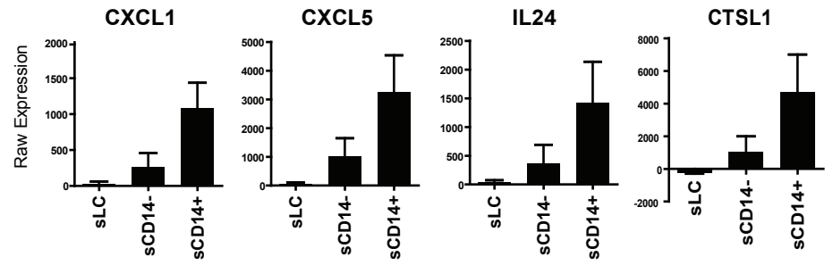
Figure S5: 6 transcripts representing 4 genes differentially expressed between the 3 skin DC subsets. a. Hierarchical clustering of the 6 transcripts differentially expressed in the 3 skin DC subsets. b. Bar charts representing the mean raw expression value for 4 of the 6 transcripts. Bars represent the standard deviation.
