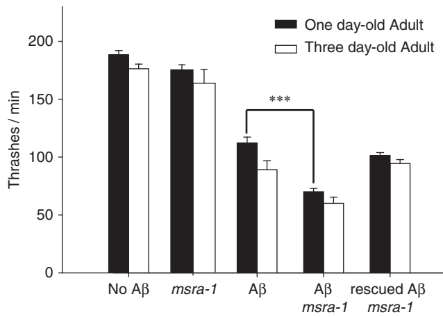
SUPPLEMENTARY FIG. S1. The deletion of the msra-1 gene worsens the locomotory impairments of Aβ transgenic worms during different ages of adulthood. The graph shows the quantification of movement in liquid medium (thrashes per minute) of 1-day-old and 3-day-old adult worms. Data are means ± SE from at least 45 animals per strain. Student's t -test was used for statistical analysis. *** p \leq 0.0001
