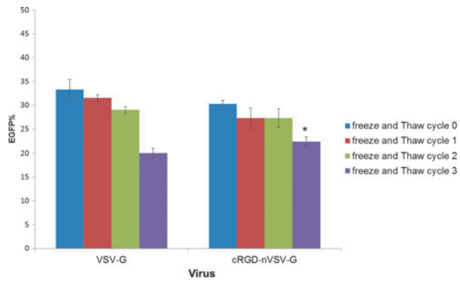
SUPPLEMENTARY FIG. S4. Stability of the targeting nanovirus after freeze–thaw cycles. VSV-G pseudotypes and the targeting nanovirus were subjected to freeze–thaw cycles (1, 2, 3), then the viruses were used to infect 1 \times 10^5 HeLa cells for 4 hr. EGFP expression was monitored by flow cytometry 3 days post transduction (* p < 0.05 ).
