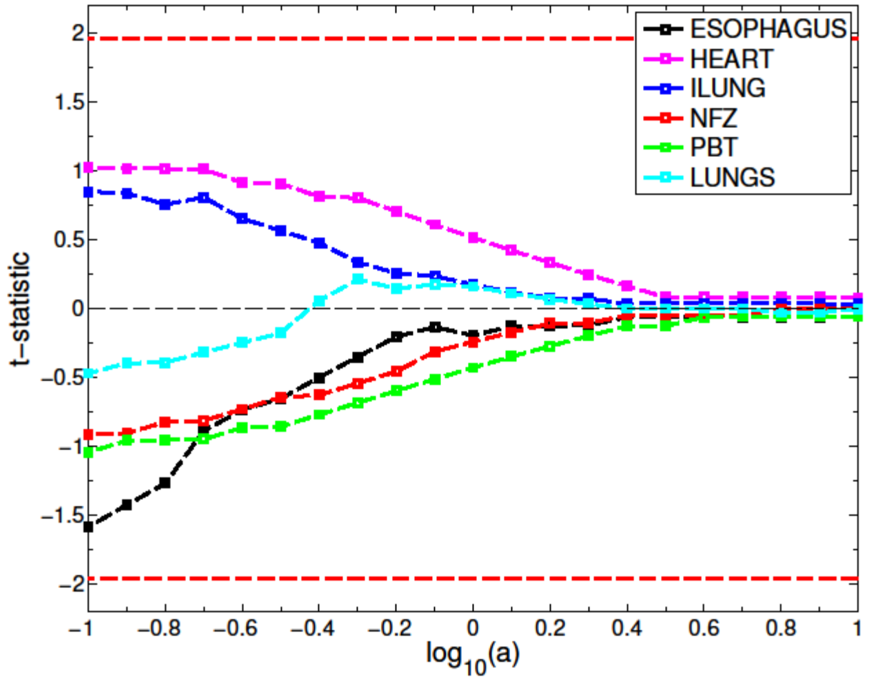
FIGURE EA3.1. T statistic values of the fitted logistic regression coefficients at each \log_{10}(a) for the ipsilateral lung, esophagus, heart, no fly zone, proximal bronchial tree, and bilateral lung dose in comparison to grade 2 or greater pulmonary toxicity. The red dashed lines show the t values corresponding to a p-value of 0.05. The sign of the t-statistic indicates the direction of the model fit (i.e. correlated or anti-correlated).
