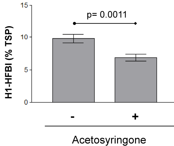
Figure S3. Impact of acetosyringone in the infiltration medium on HA-HFBI accumulation.
