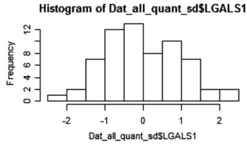
SUPPLEMENTARY FIG. S3. Distribution of Ct values per gene.
