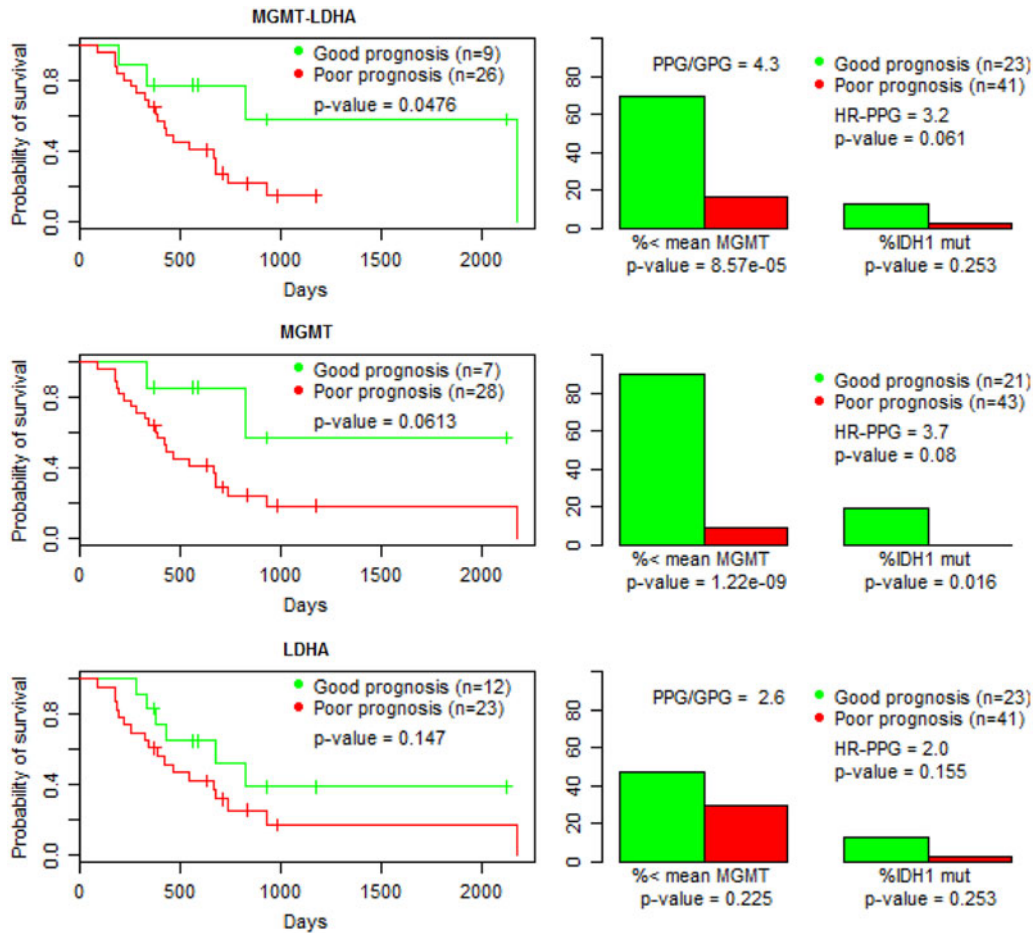
SUPPLEMENTARY FIG. S8. Survival and molecular features of LDA functions based on classification obtained from microarrays experiments for the 25 training cases. The test cases ( n=39 ) were classified as group of good and poor prognosis (GPG and PPG) using Equations 3–5, while the original label obtained from Supplementary Fig. S5 above was set to the training cases ( n=25 ). Left plots are survival curves based on LDA functions fitted with either MGMT-LDHA , MGMT , or LDHA expression values. All samples having survival data available were used ( n=35 ). The p value indicates the probability that curves are equal. Plots on the right depict the percentage of cases showing an MGMT expression below the average of all cases ( n=64 ) and the percentage of cases showing an IDH1 mutation in each group (GPG and PPG). The p value denotes the probability that proportions are equal.
