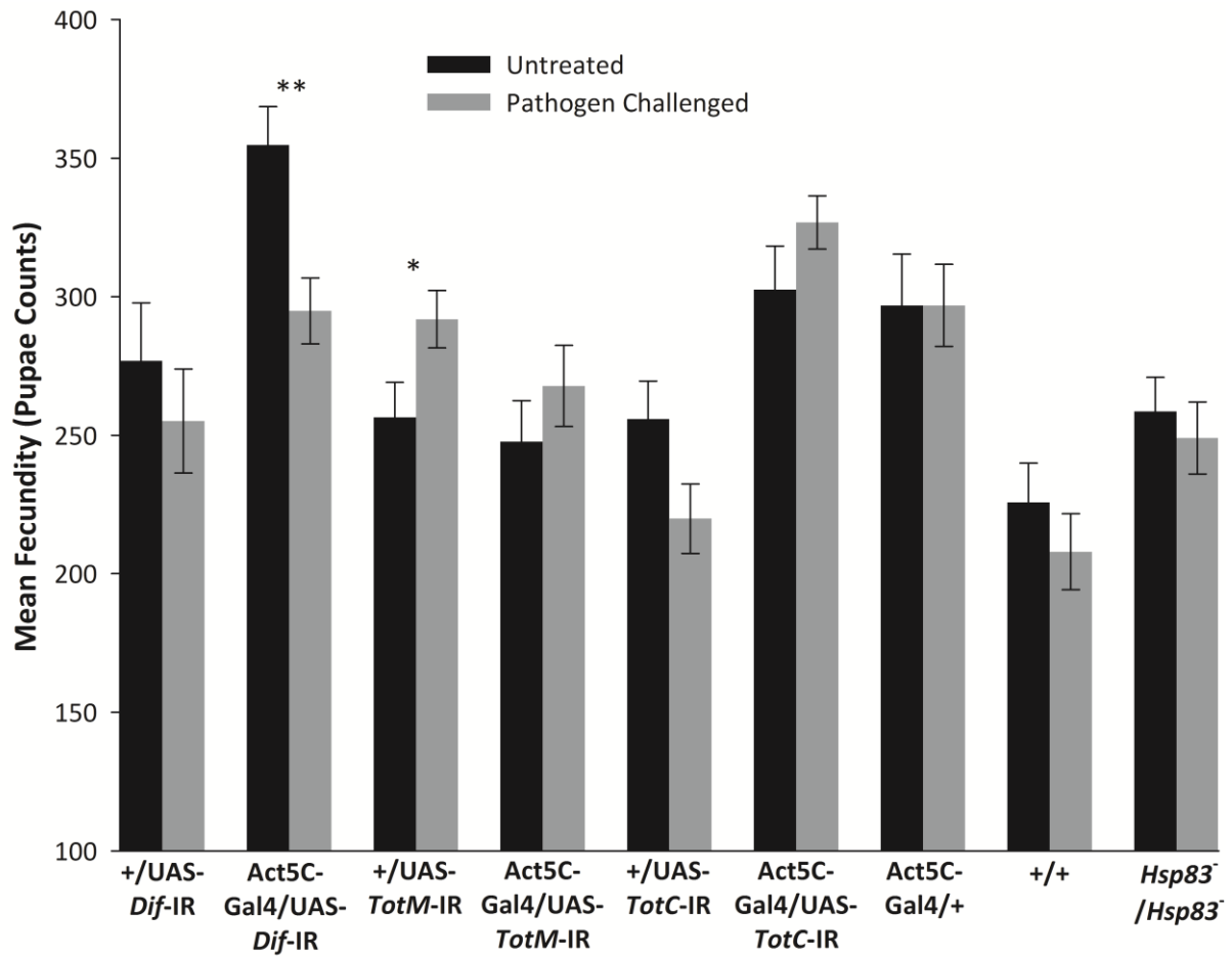
Supplementary Figure 3: Mean fecundity of each genotype. Black indicates flies treated with a sham treatment (control) and grey indicates flies treated with heat-killed fungal spores ( \pm SE). Average fecundity was taken from pupae counts over 10 day samples. * - P < 0.05 , ** - P < 0.01
