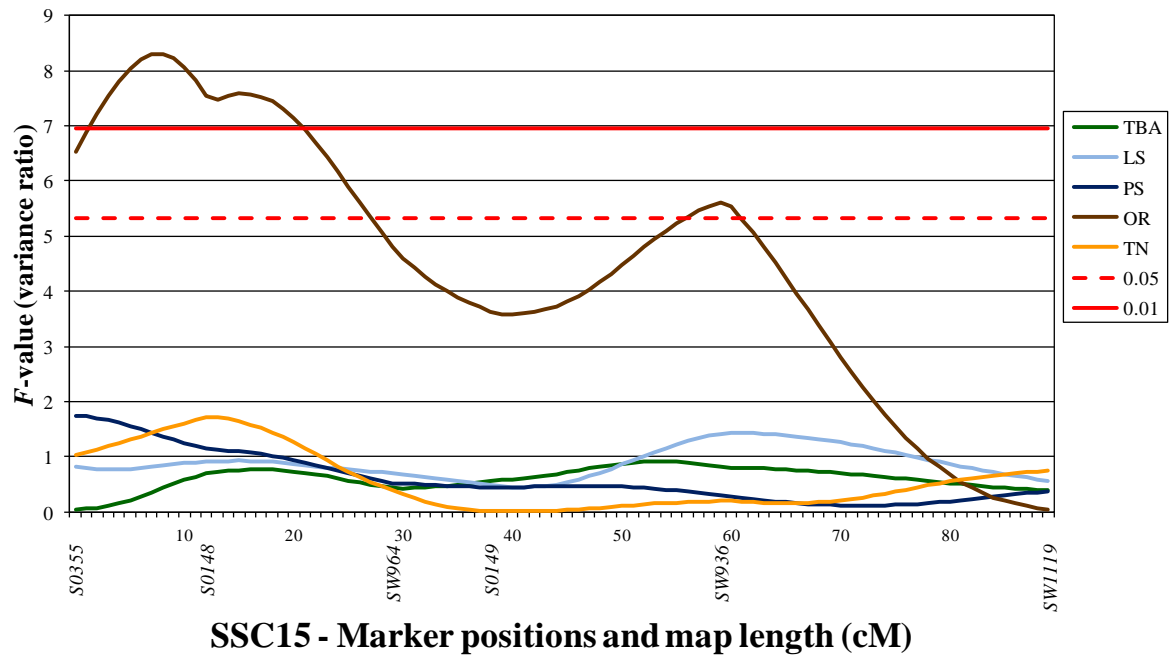
Figure S6 Interval mapping for QTL with effects on TBA, LS, PS, OR and TN on SSC15. Chromosome-wide significance level at P < 0.05 (broken red line) and P < 0.01 (solid red line). TBA, total born alive; LS, litter size; PS, prenatal survival; OR, ovulation rate; TN, teat number.
