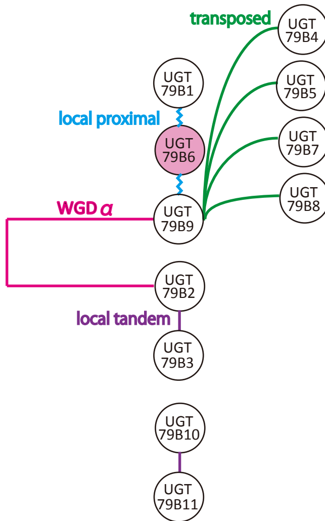
Figure S7. Modes of gene duplication in Arabidopsis UGT79 subfamily. The gene duplication modes proposed by Wang et al., 2013 were shown (Wang et al., 2013). WGD, whole genome duplication.
