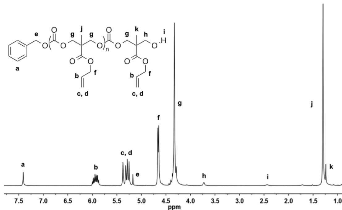
Fig. S2 ^1\text{H} NMR spectrum of BnO-PMAC 15 -OH initiated from benzyl alcohol using DBU. Conditions: [MAC] 0 = 0.5 M in DCM a 29 °C in the glovebox, [MAC] : [BnOH] : [DBU] = 20 : 1 : 1.
