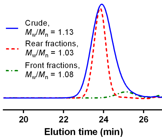
Fig. S3 GPC profiles (THF as eluent, 1 mL/min) of BnO-PMAC 15 -OH before and after purification using column chromatography. Conditions: [MAC] 0 = 0.5 M in DCM at 29 °C in the glovebox, [MAC] : [BnOH] : [DBU] = 20 : 1 : 1.
