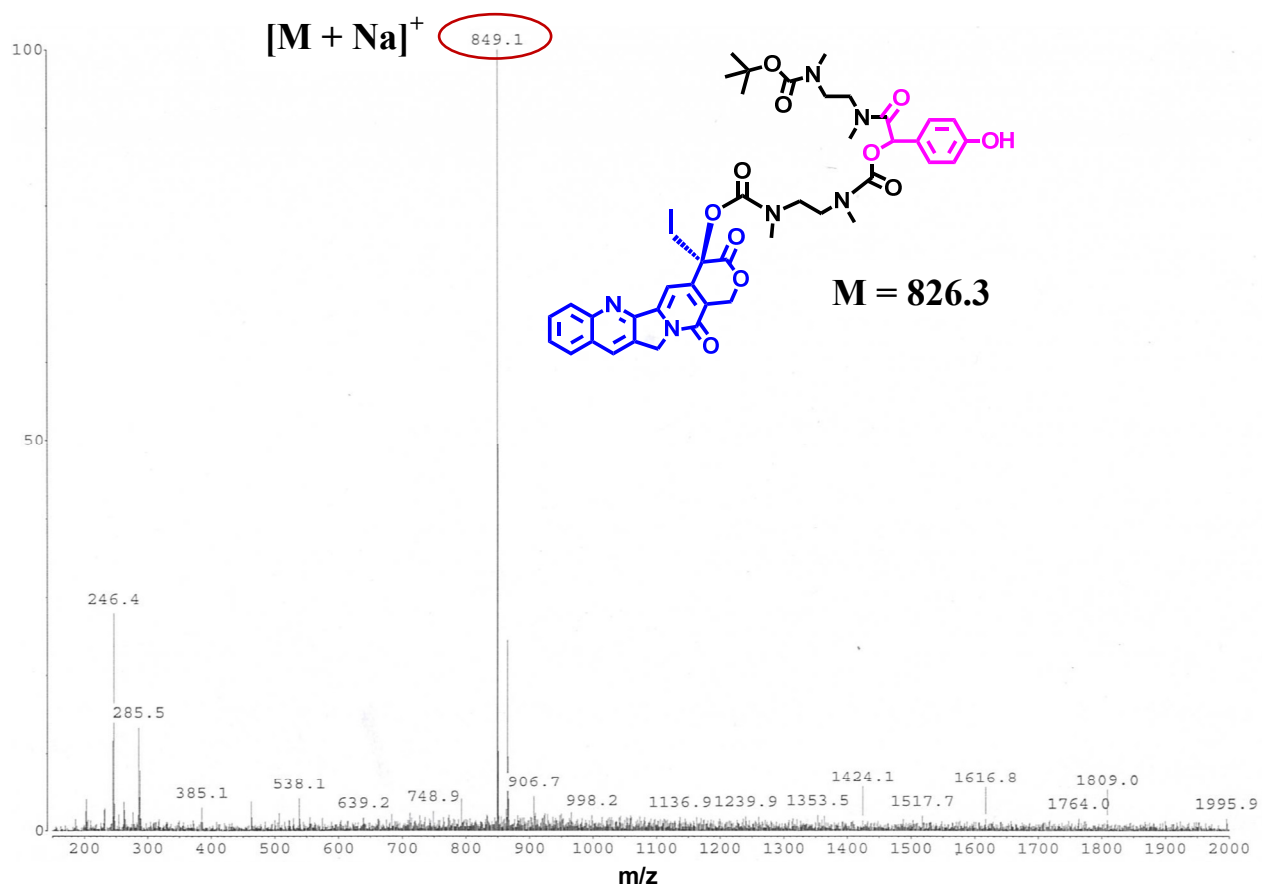
Mass spectrum of CAS-CPT immediately after photoirradiation (365 nm, 2.5 mW/cm 2 , 10 mins).
