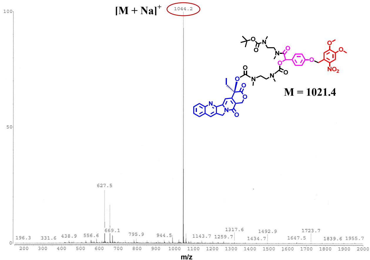
Mass spectrum of compound 7 (CAS-CPT).
