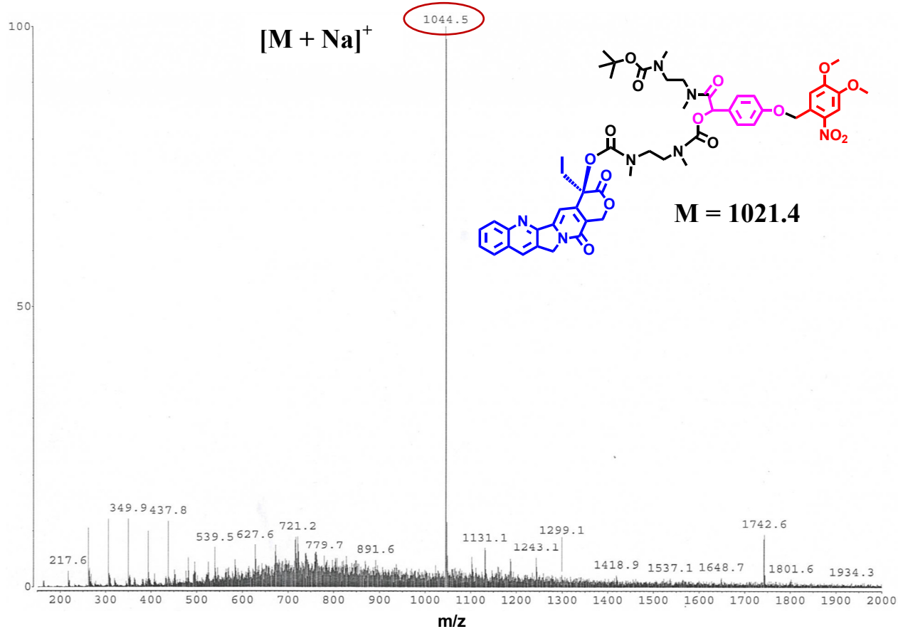
Mass spectrum of CAS-CPT before photo-irradiation.
