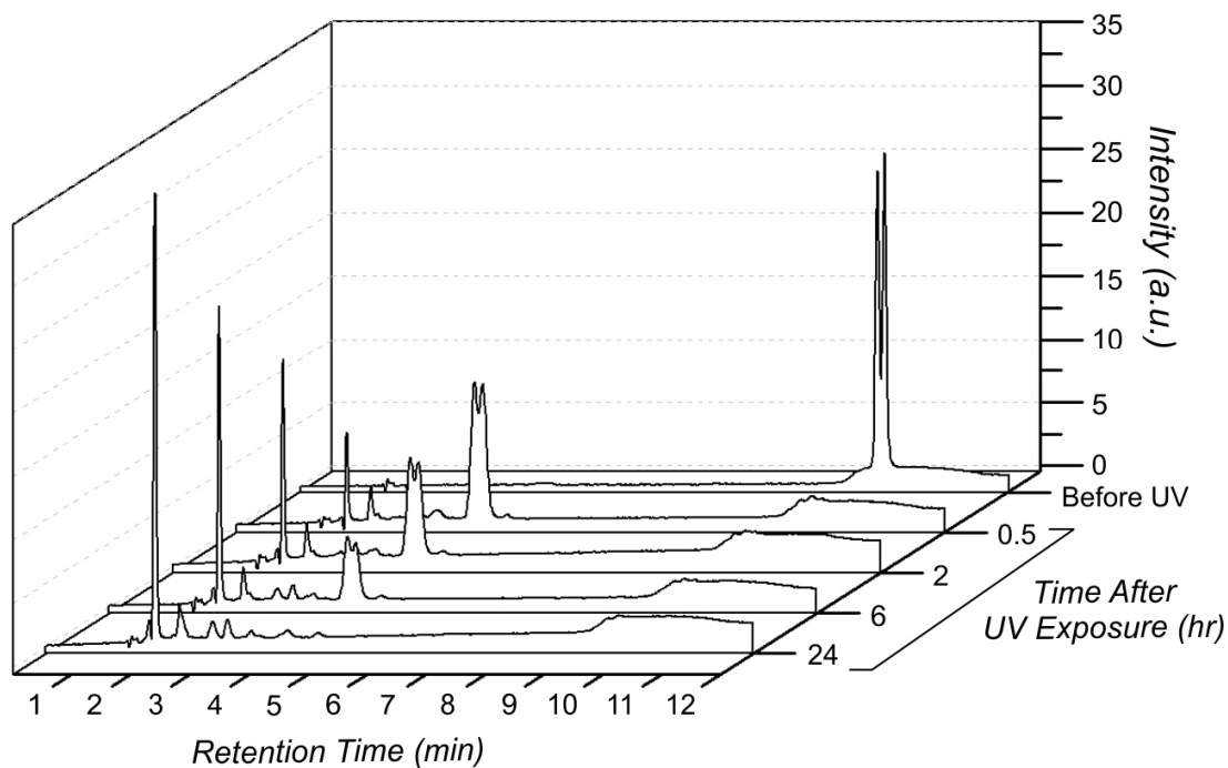
Figure S1. HPLC Chromatograms showing CPT release over time from CAS-CPT after photoirradiation. CAS-CPT (20 \mu\text{M} ) was dissolved in aqueous medium (1xPBS containing 2% DMF). The solution was exposed to UV light (365 nm, 2.5 \text{mW}/\text{cm}^2 ) for 10 mins and then monitored over 24 hrs.
