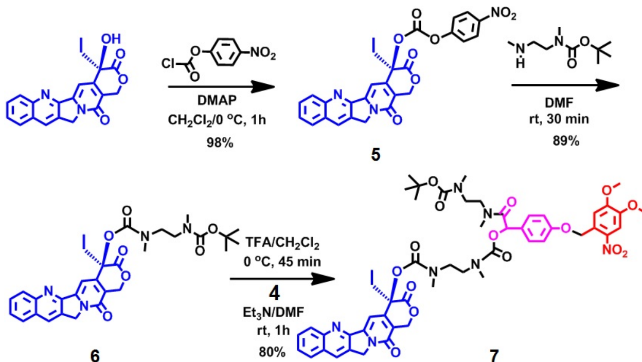
Scheme 2. Synthetic scheme for conjugation of camptothecin (CPT) with chemical adaptor system (CAS) [CAS-CPT].
