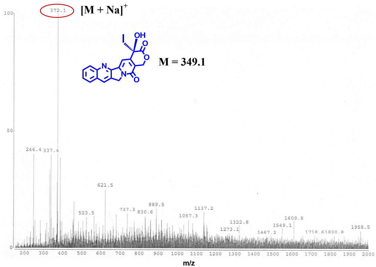
Mass spectrum of CAS-CPT 24h after photoirradiation.
