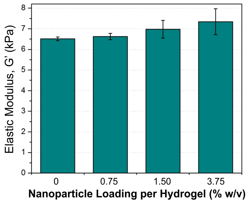
Figure S3. Elastic moduli of hydrogels with varying loadings of NP-CAS-CPT. Rheometry measurements were acquired at a 0.1% shear rate and the moduli reported at a 1 Hz frequency.
