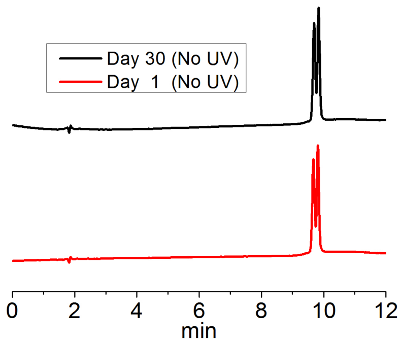
Figure S2. HPLC Chromatograms showing stability of CAS-CPT in 1xPBS in the absence of photo-irradiation, monitored over 30 days.
