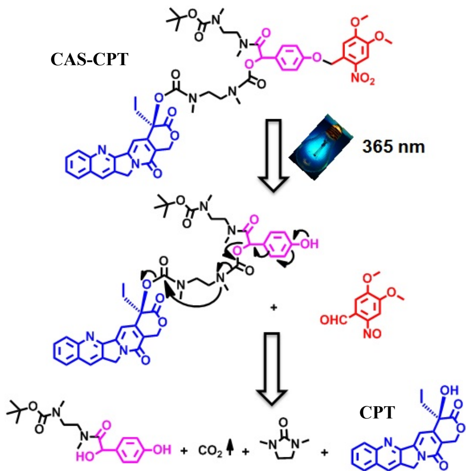
Scheme 3. Proposed Mechanism of Drug Release from CAS-CPT.
