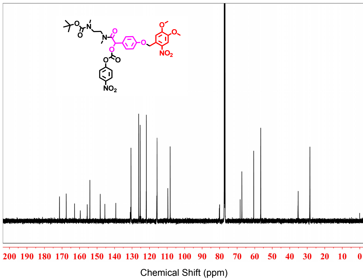
^{13}\text{C} NMR of compound 4 in \text{CDCl}_3 .
