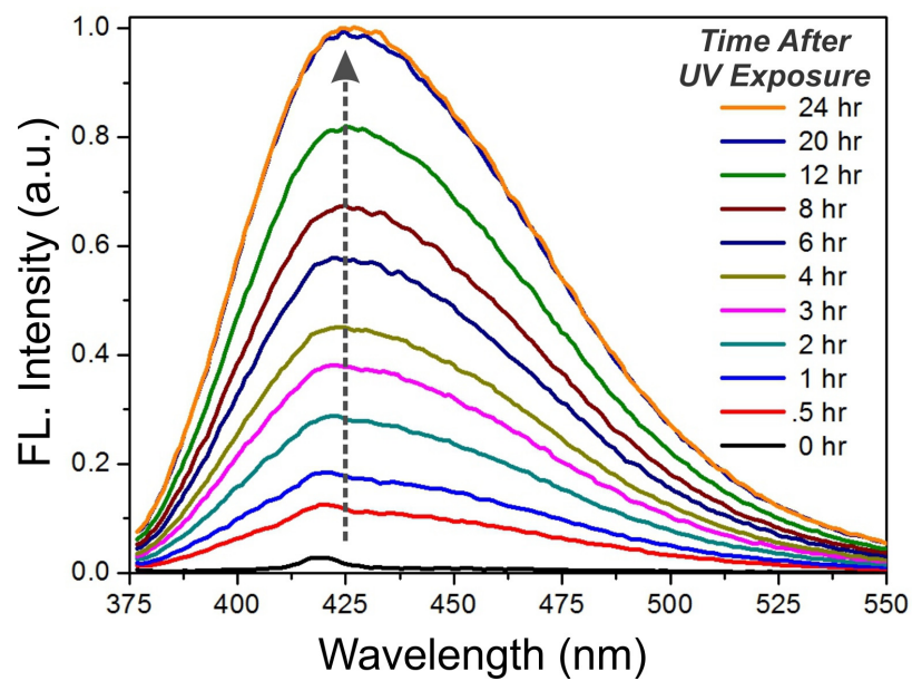
Figure S4. Fluorescence emission spectra of CPT release from hydrogel-NP hybrid scaffolds. The emission spectra ( \lambda_{\text{ex}} = 368 \text{ nm} ) was monitored over 24 hrs after 10 min irradiation with UV light ( 365 \text{ nm} , 2.5 \text{ mW/cm}^2 ).
