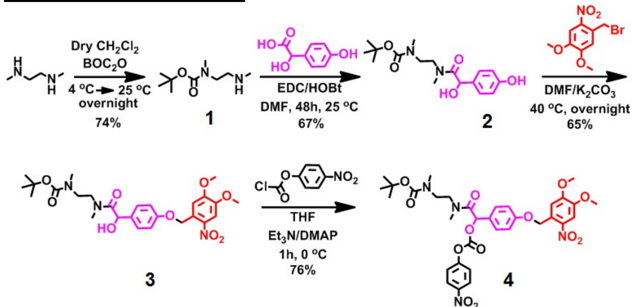
Scheme 1. Synthetic scheme for chemical adaptor system (CAS).
