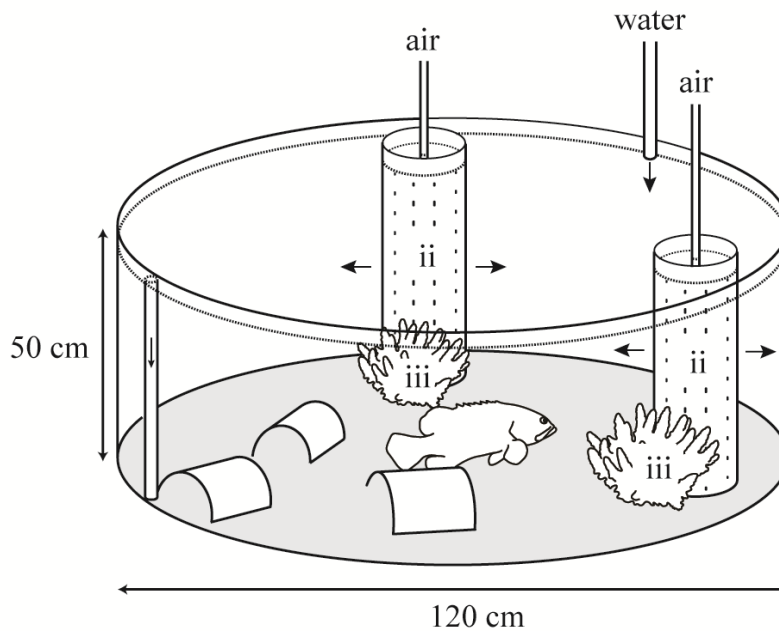
Figure S2. Diagrams of tank setups. a) shows the setup for the nocturnal olfactory trials using coral-dwelling crabs. A filefish or coral fragment was placed into each perforated tube (i). b) shows the setup for trials using predatory cod. A filefish fed a specific diet was placed into each of the perforated tubes (ii). Depending on the treatment, a specific coral was placed next to each perforated tube (iii). Arrows indicate water movement, as confirmed from dye trials.
