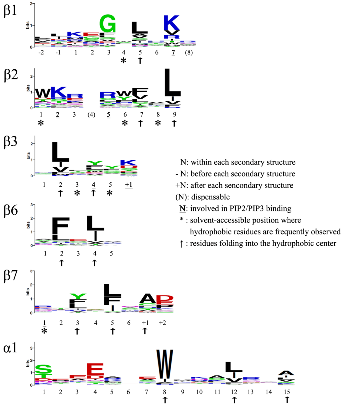
Figure S1. Sequence logos for PH domain. Position-specific logos for the secondary structure elements of PH domain (generated by Weblogo server). \beta_4 and \beta_5 are not included because of the high variation within these two \beta -sheets. The size of residue indicates the relative frequency of the residue at the corresponding position.
